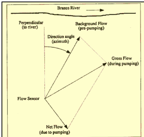
Figure 7. Plan view of the ground water flow vector subtraction convention used for derivation of net flow in the analysis of flow sensor and piezometric data. The direction (azimuth) convention is also shown.
