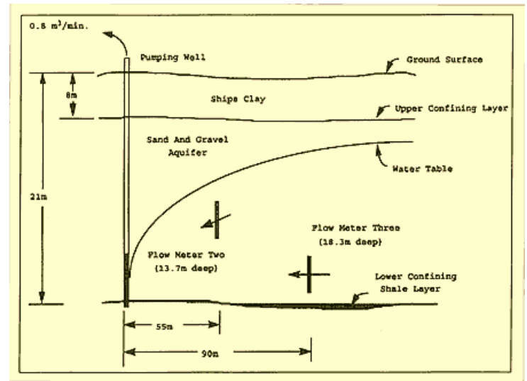
Figure 3. Elevation view of the pumping well and the 3-D flow sensors at the Brazos River Site with soil stratigraphy also shown (not to scale).
