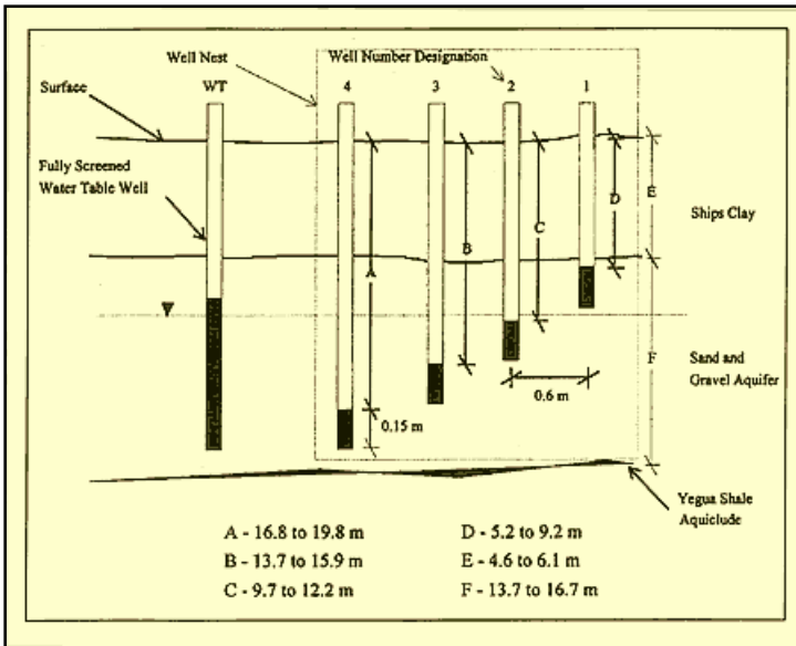
Figure 2. Elevation view of a typical well nest and water table well soil stratigraphy and range of piezometer well screen depths shown (not to scale).
